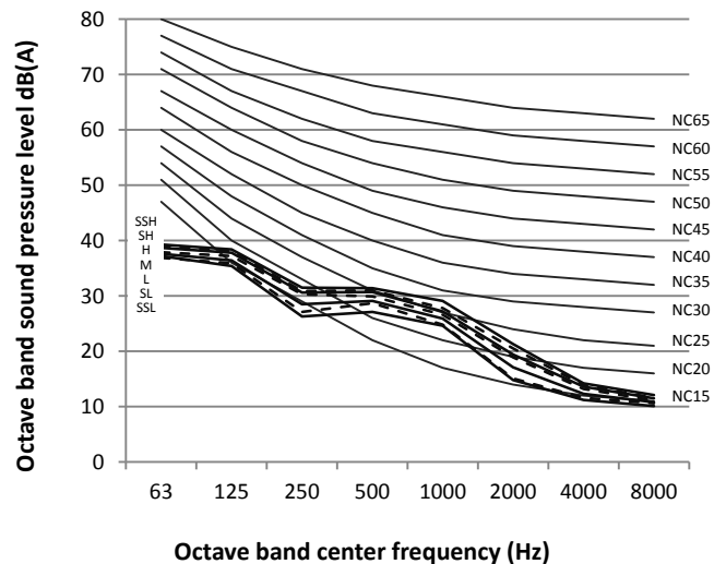
Figure 8.3: MI2-36GDN1 octave band levels
