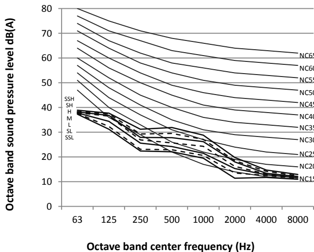
Figure 8.2: MI2-22(28)GDN1 octave band levels
