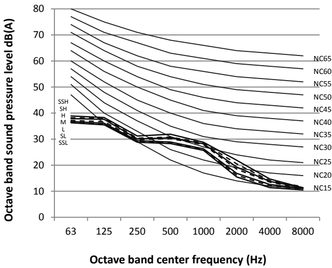
Figure 8.6: MI2-71(80)GDN1 octave band levels
