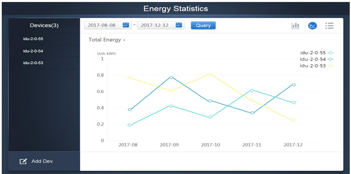
(Line Graph)
