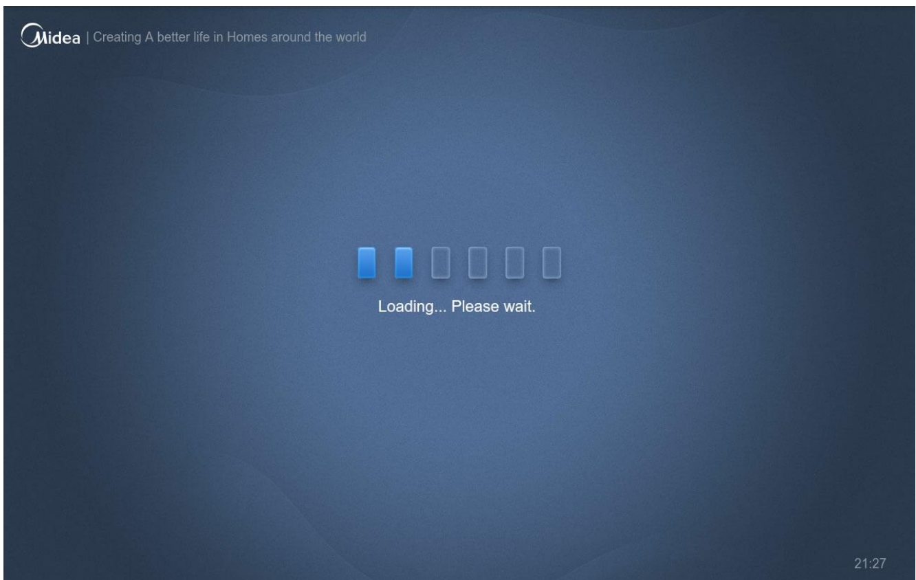
(Boot Screen)
