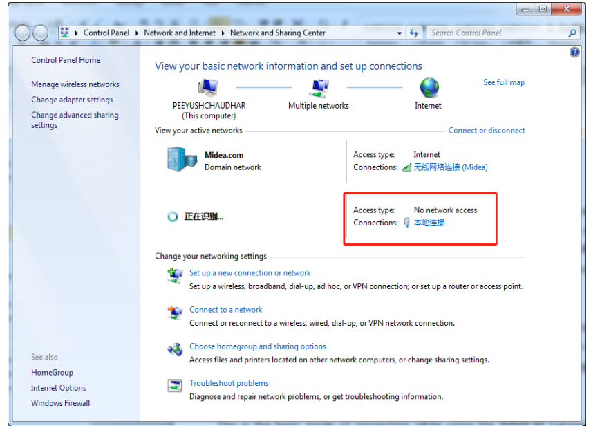
(Dialog box 2)
