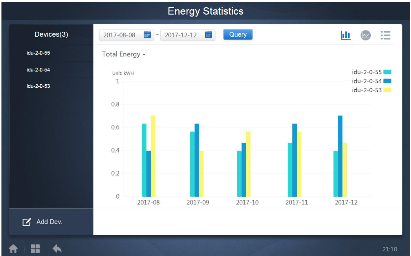
(Histogram)
