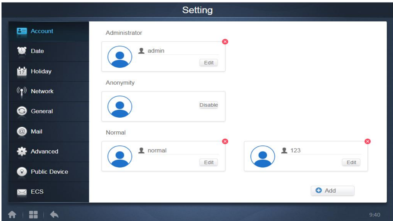
(Administrator Page)
