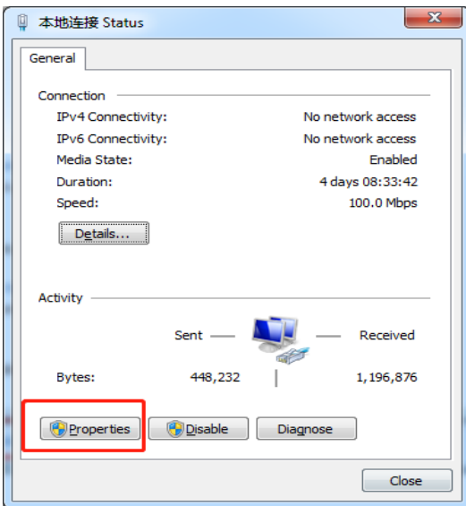
(Dialog box 3)
