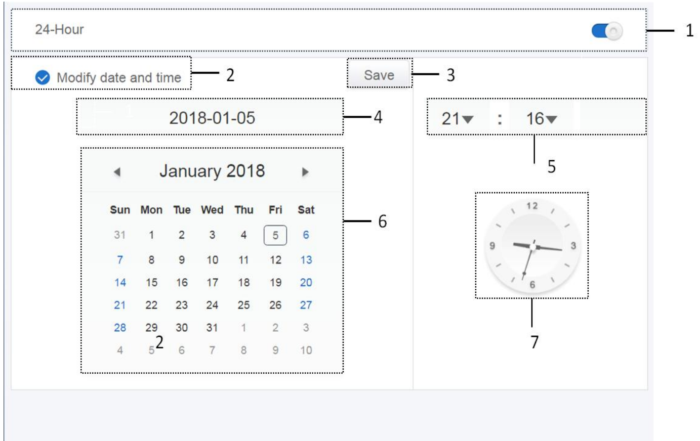
(Edit Mode)
